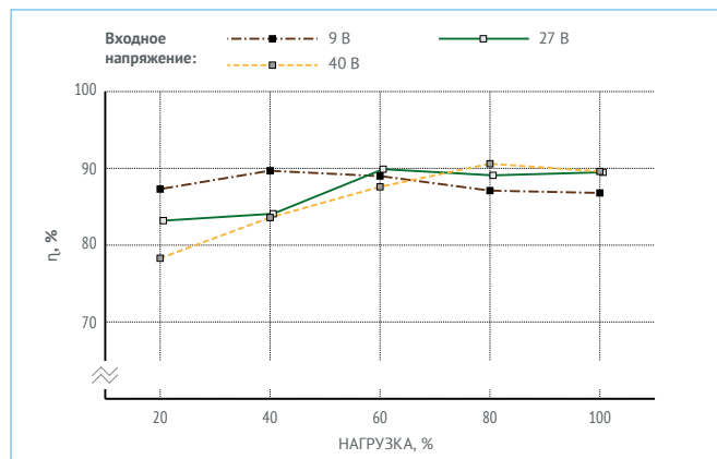
Рис. 11. МДМ50-1B09PDS.
